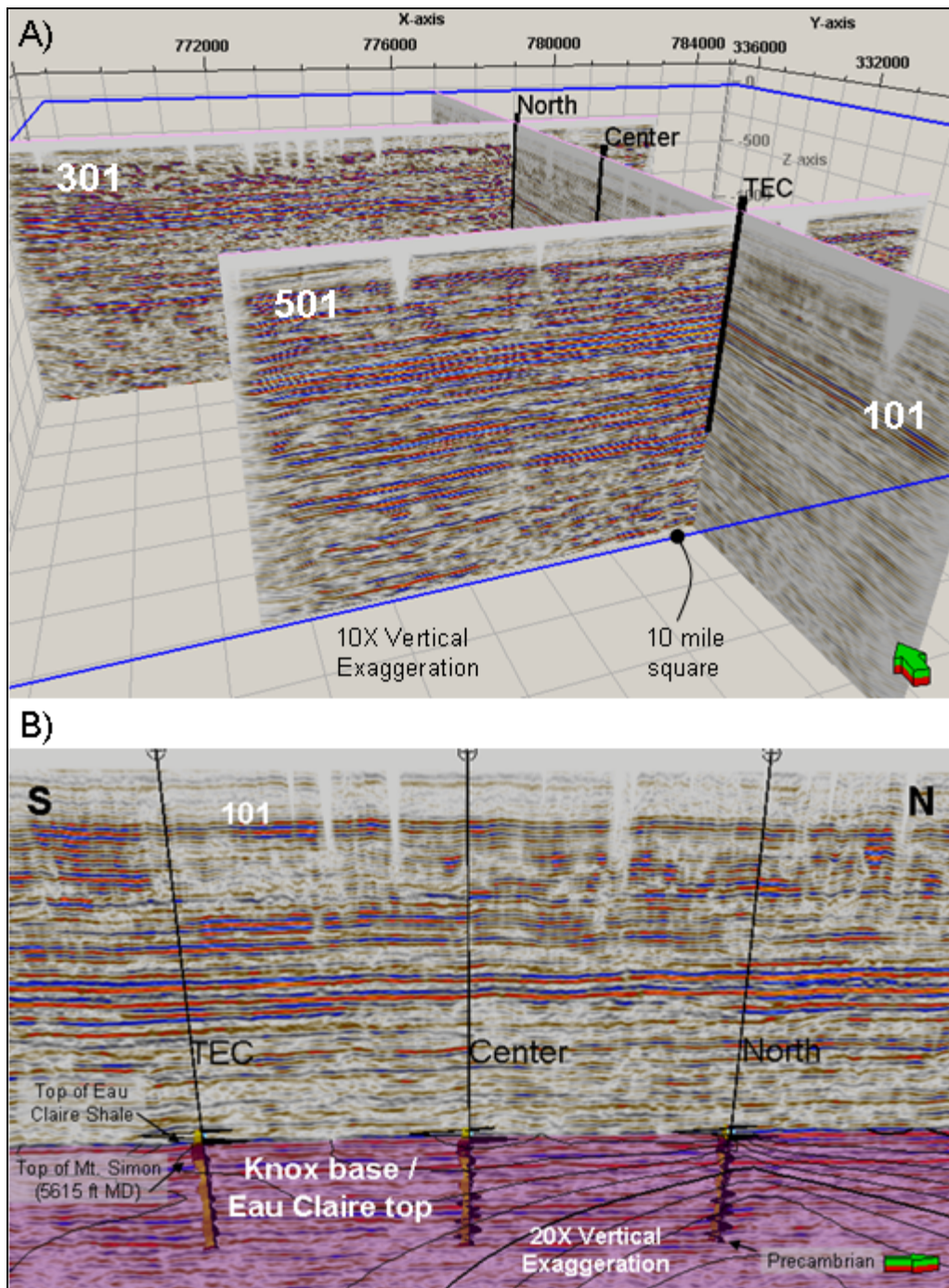
Figure 3. The three 2D seismic lines are shown here adjacent to the three proposed injection wells. A) The three proposed injection wells are placed 2 miles apart. The blue line represents a square with 10-mile-sides centered on the proposed “Center” well. B) Gamma ray logs and synthetic seismograms based on sonic logs are used to interpret the contact between the base of the Knox dolomite and the Eau Claire shale. The Mt. Simon is deeper at 5615 feet.
