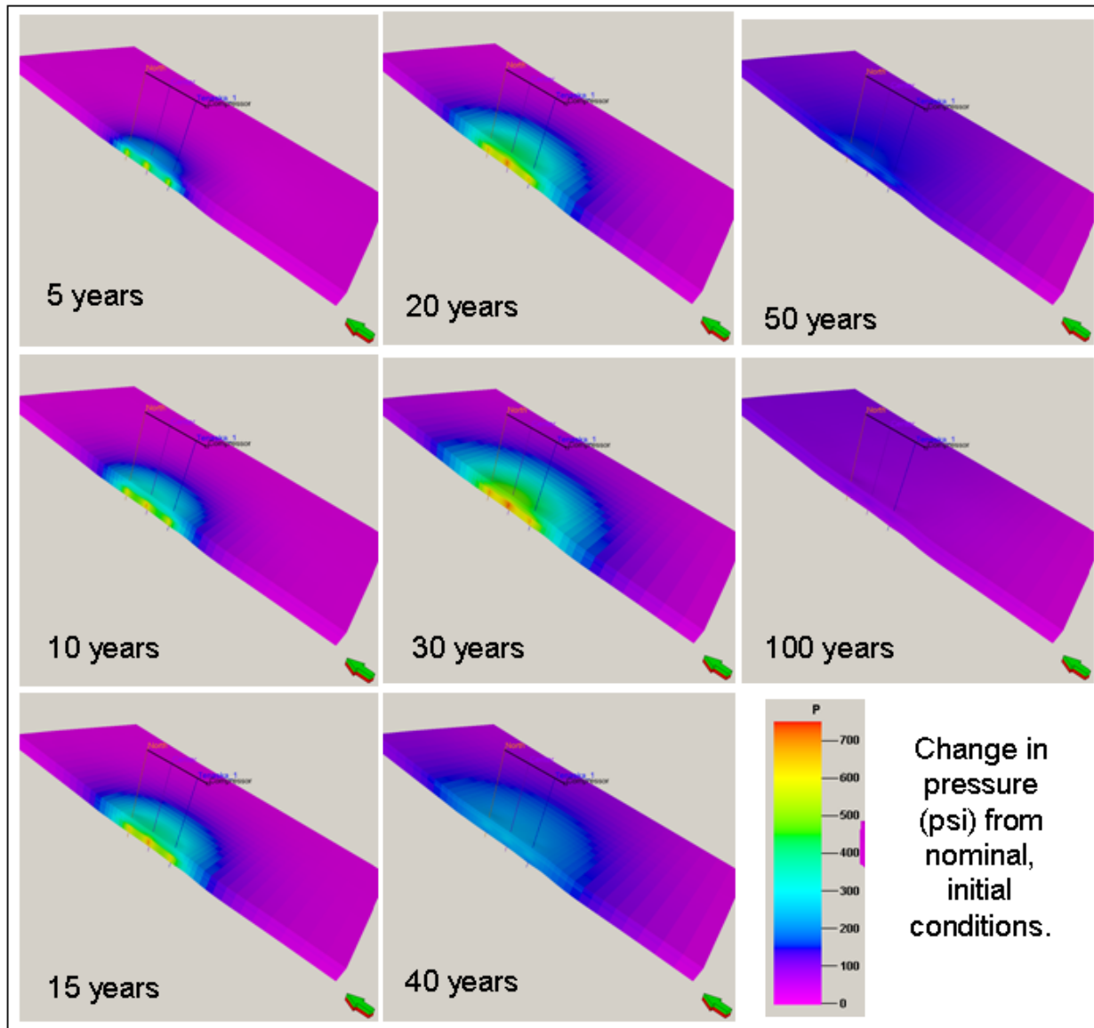
Figure 6. Oblique, cut-away view of the Mt. Simon reservoir model showing the three injection wells and changes in reservoir pressure through time. Change in reservoir pressure is shown relative to the start date of the simulation of January 2010. After the 30 years of injection, the pressure begins to declines back to initial conditions.
