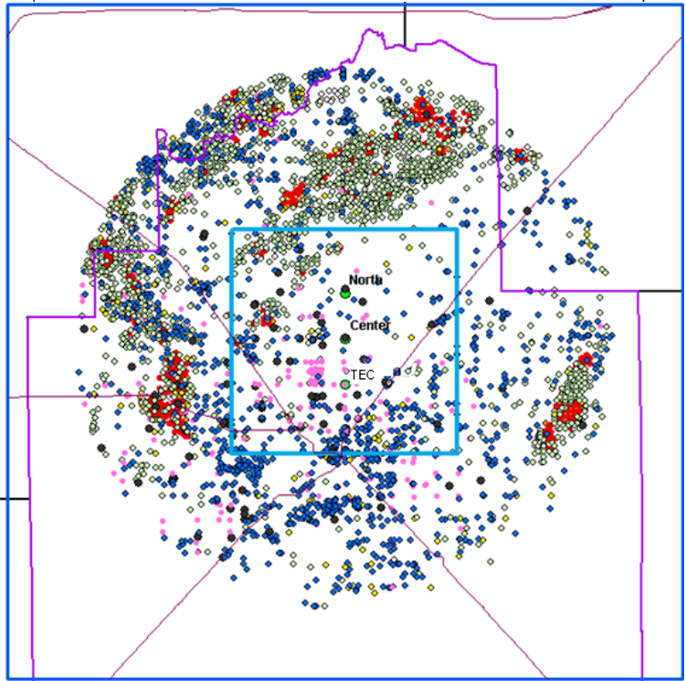
Figure 2. Near-surface features in the study area include coal mines and wells. The Herrin Coal seam exists throughout Cristian County and has been mined locally. An inventory of wells in a 12-mile radius of the proposed Center well reveals the presence of some hydrocarbons. These resources are relatively small, and more importantly, shallower than the intended CO 2 storage interval.
