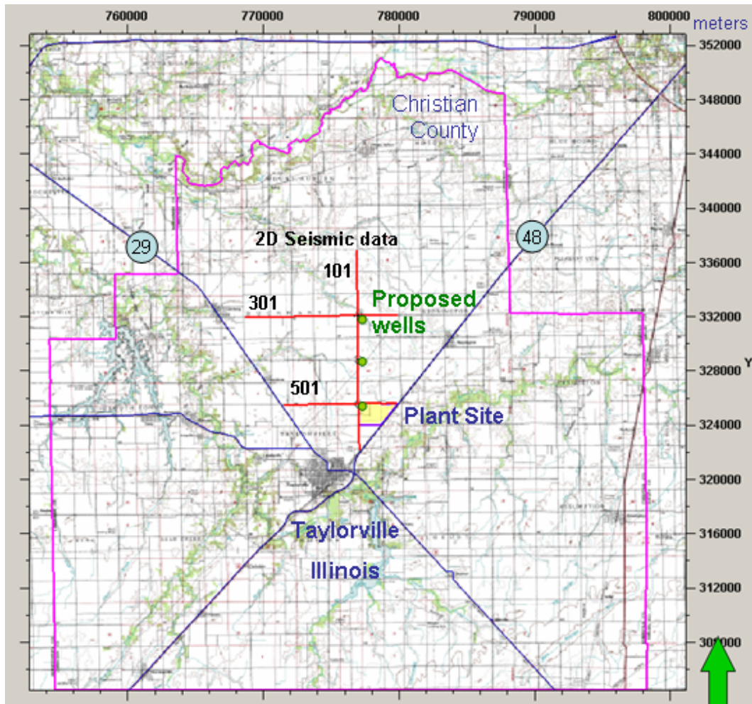
Figure 1. Topographic map of the 30x30 mile study area. The proposed plant site is located a little over two miles northeast of Taylorville Illinois along State Route 48. Located in Christian County, north of Taylorville, three proposed injection wells are shown here adjacent to three 2D seismic lines that were acquired in July 2009.
