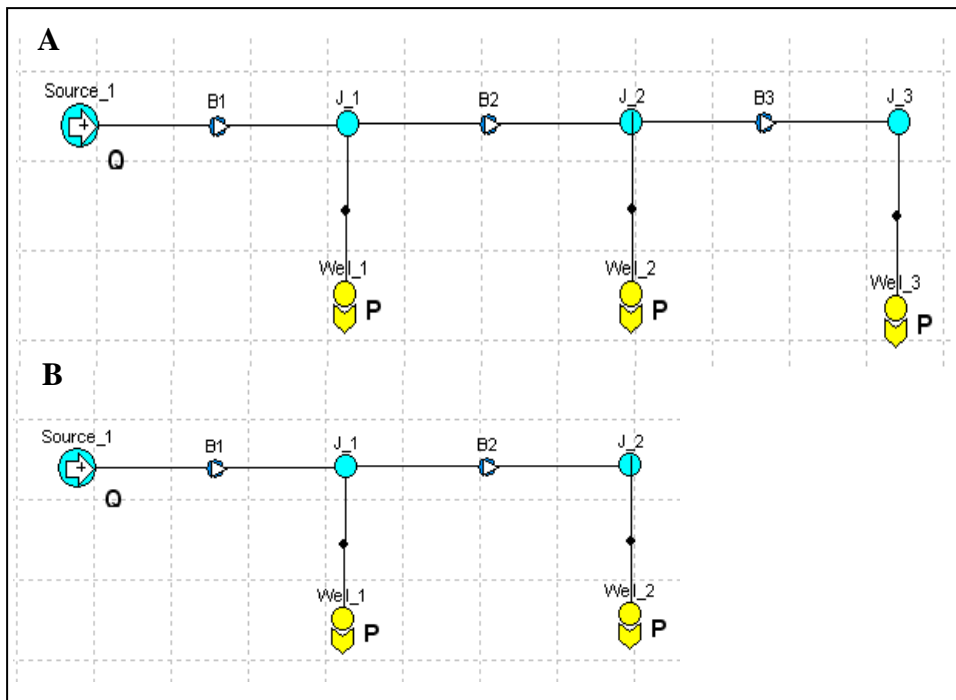
Figure 5. Pipeline networks for the 5.5-inch (A) and 7-inch (B) injection wells used in the PIPESIM modeling.
