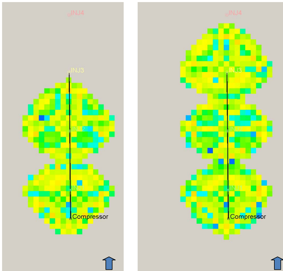
Figure 8. Comparison of reduced injection in two wells to full injection in three wells.
