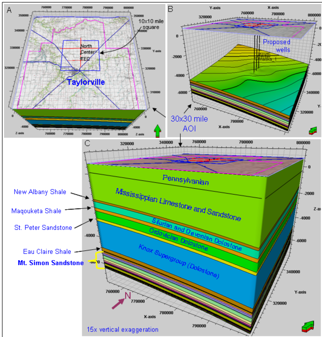
Figure 4. Geological model for a 30x30 mile Area of Interest (AOI) around the TEC site. The reservoir model consists of 27 Mt. Simon zones and 264 layers. The initial model consists of 6.7 million cells that are 300 meters square. A) Oblique map view of the proposed TEC wells north of Taylorville, Illinois. B) Cut-away view of the model showing the proposed wells penetrating the top of the Eau Claire Shale. Based on 2D seismic data, the strata dips to the southeast by less than one degree. C) Layer cake geological model illustrating some of the key reservoirs and seals within the Area of Interest. Note the dip to the southeast. The Mt. Simon portion of the model is refined with many layers to realistically represent the natural petrophysical variations in the formation.
